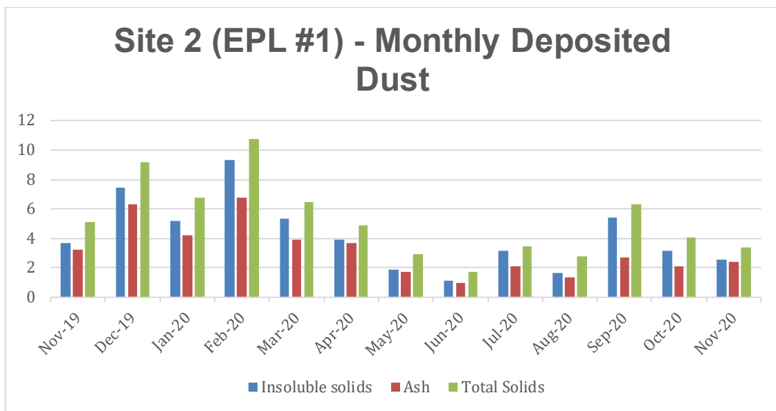
Figure 9 - Widemere Recycling monthly deposited dust results for Site 2
